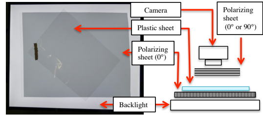
Figure 6: Photoelasticity effects produce colors in transparent plastics placed between two polarizing sheets.
